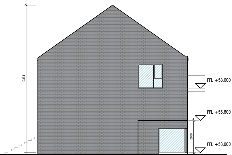
LHS ELEVATION SCALE 1:200
