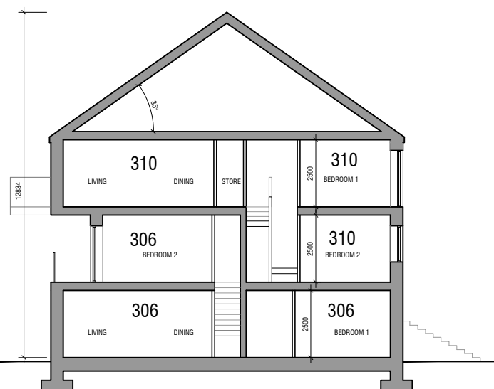
SECTION SCALE 1:200
