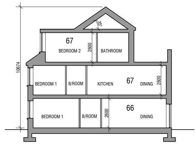
SECTION SCALE 1:200
