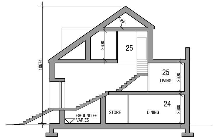
SECTION SCALE 1:200
