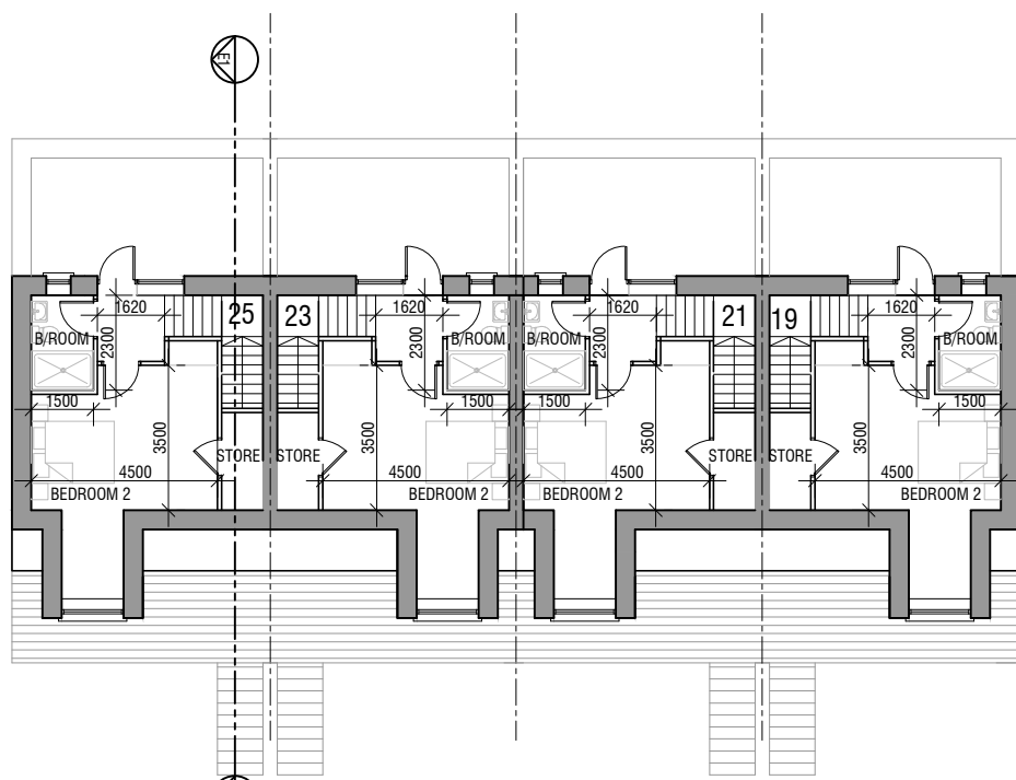
SECOND FLOOR PLAN - TYPE E1 SCALE 1:200
