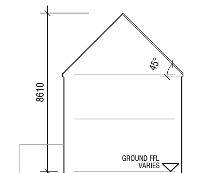
SIDE ELEVATION D3 SCALE 1:200
