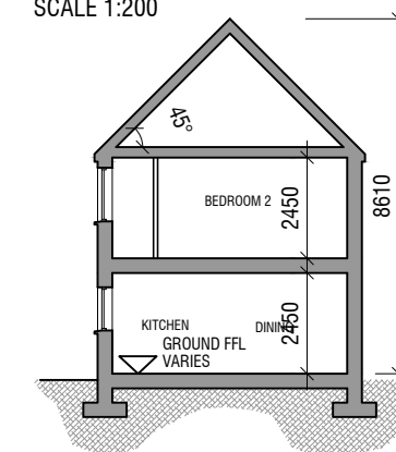
SECTION D3 SCALE 1:200
