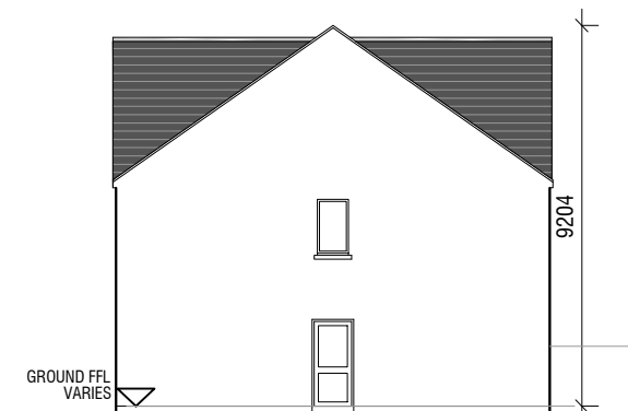
SIDE ELEVATION C22
