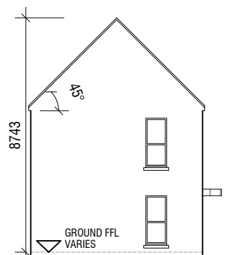
SIDE ELEVATION C5 SCALE 1:200
