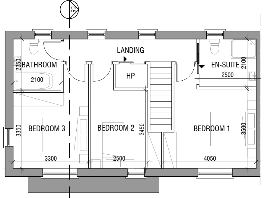
FIRST FLOOR PLAN C5 SCALE 1:100
