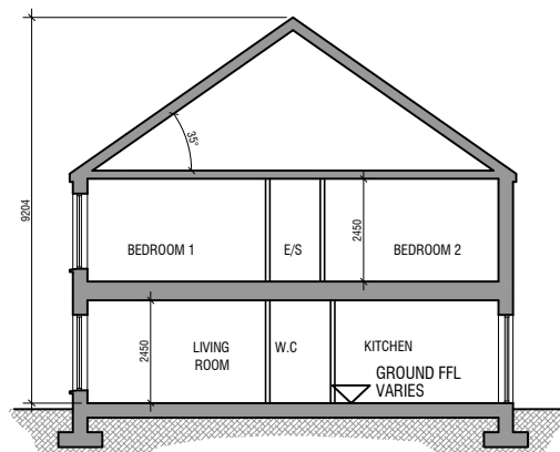
SECTION C3 SCALE 1:200
