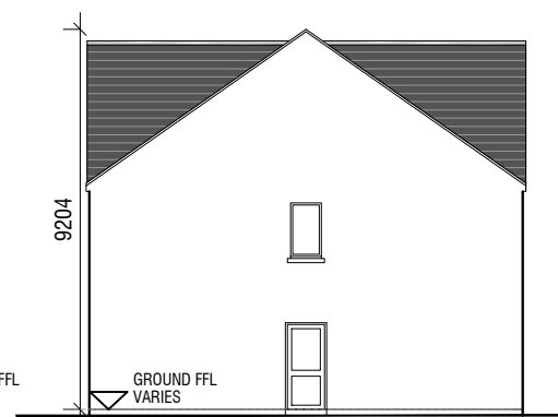
SIDE ELEVATION C3.2 SCALE 1:200
