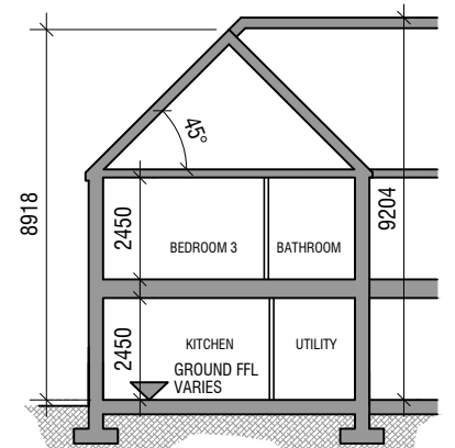
SECTION C2.3 SCALE 1:100
